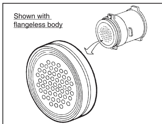
Figure 8: Lo-Noise Trim – LNA/LNB
